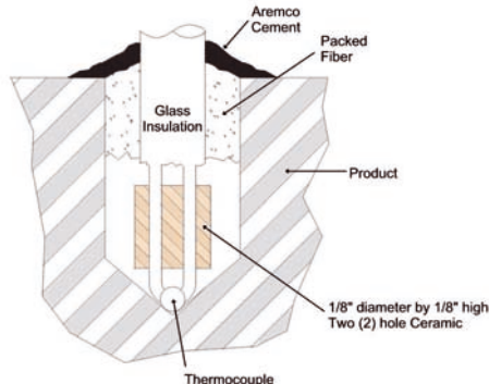
Fig. 4 Thermocouple Configuration
