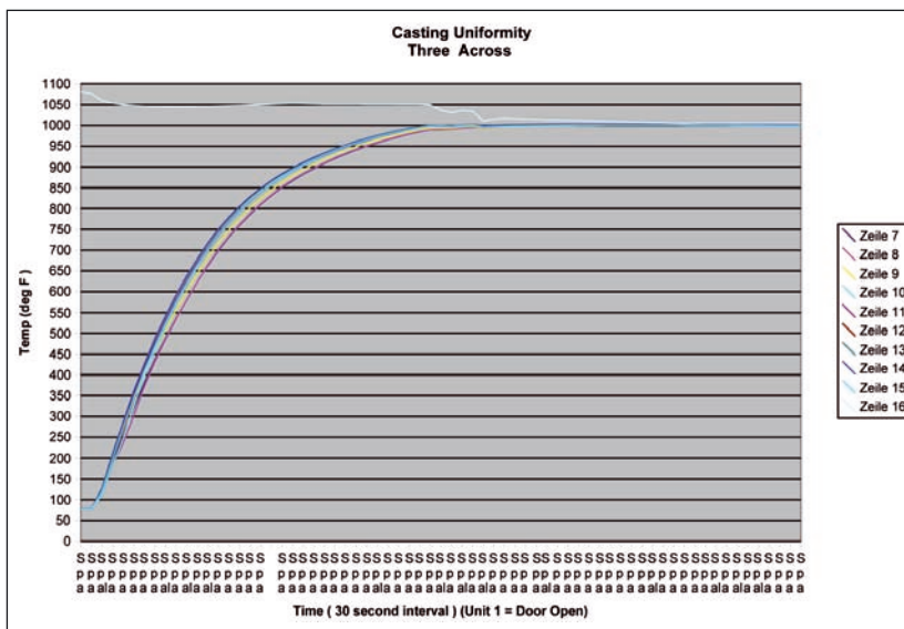
Fig. 7 Temperature vs. Time in an expanded scale beginning when all temperatures were above 995 deg. F
