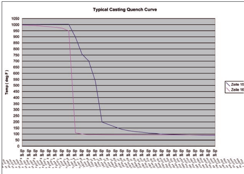
Fig. 9 Typical casting temperature and ambient temperature during the quench cycle
