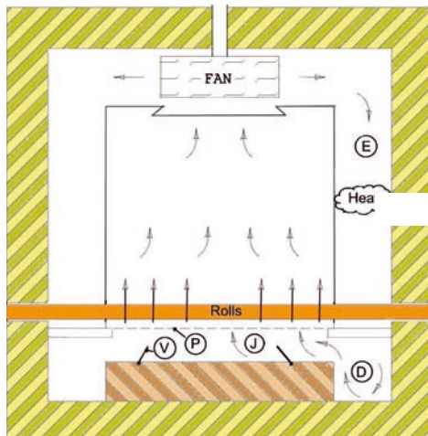
Fig. 1 Mass Flow – Jet Impingement Furnace
