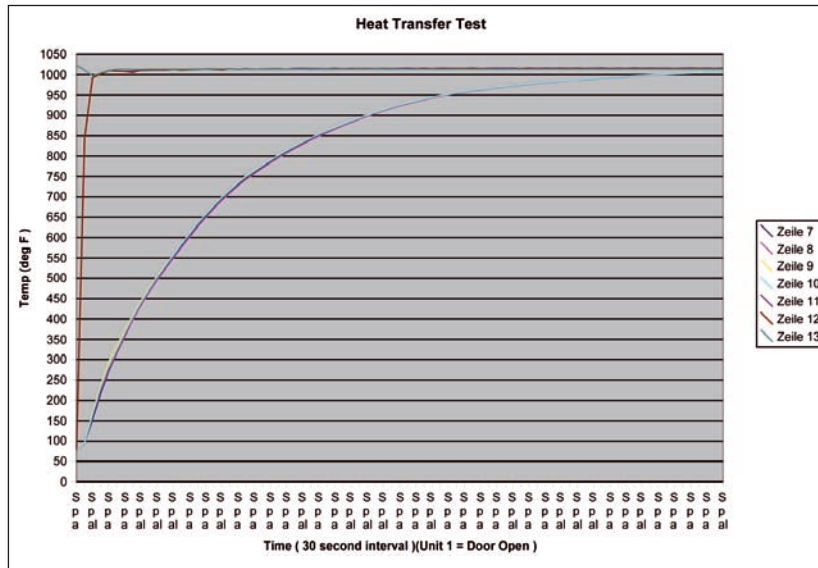
Fig. 8 Plate temperature vs. elapsed time (heating curve) for a one inch thick 6061 aluminium plate at a distance of 4-1/4 inches from the jet plate
