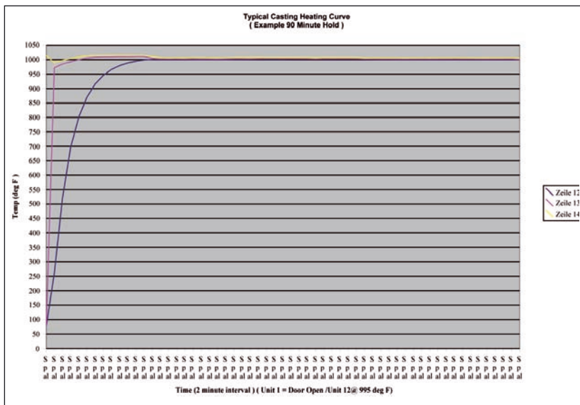
Fig. 10 Typical temperatures during the heat/hold portion of the heat treat cycle
