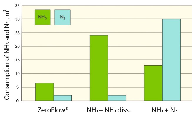
Comparison of consumption of NH 3 and N 2 in the traditional processes and ZeroFlow® during nitriding of a crankshaft made from steel 4340 (retort volume – 0.6 m³)
