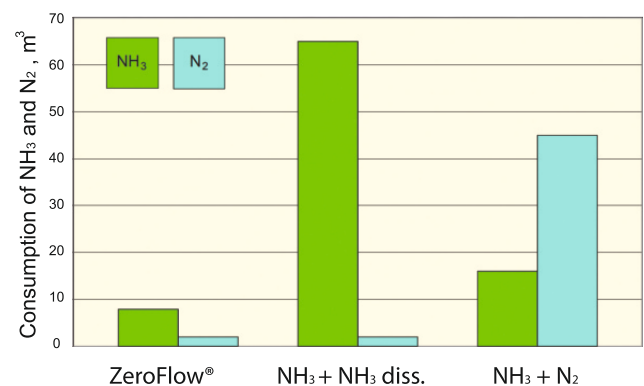
Comparison of consumption of NH 3 and N 2 in the traditional processes and ZeroFlow® during nitriding of wheels for wind power plants made from steel 31CrMoV9 (retort volume – 0.6 m³)
