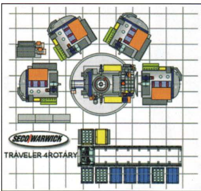
Fig. 11 — Seco/Warwick multi-chamber system (Traveler Rotary).
