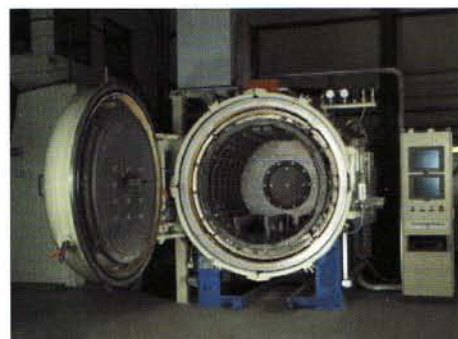
Fig. 1 -- HPQ furnace with axial/radial quenching system.
