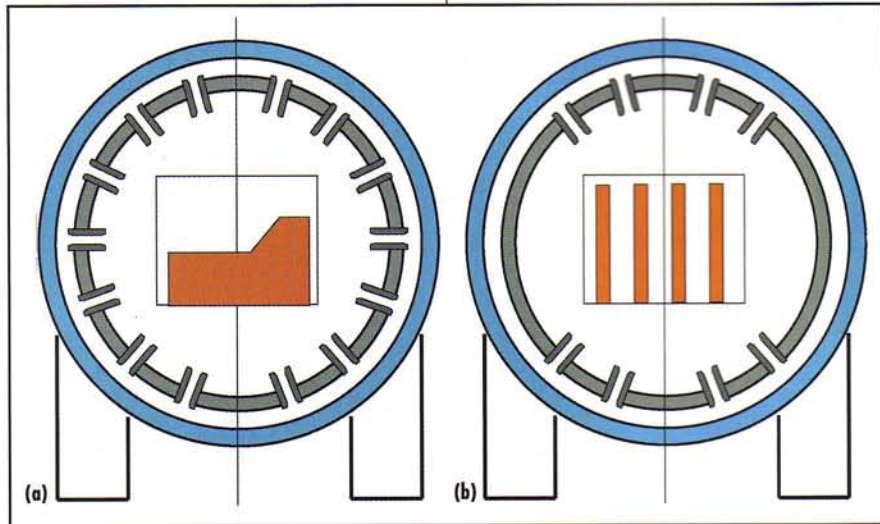
Fig. 2 — Radial gas flow (a), and axial gas flow (b).
