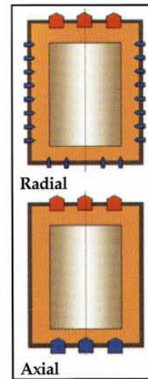
Fig. 5 — Elevator furnace (72 in. diam. × 72 in. high) with axial/radial quenching.
