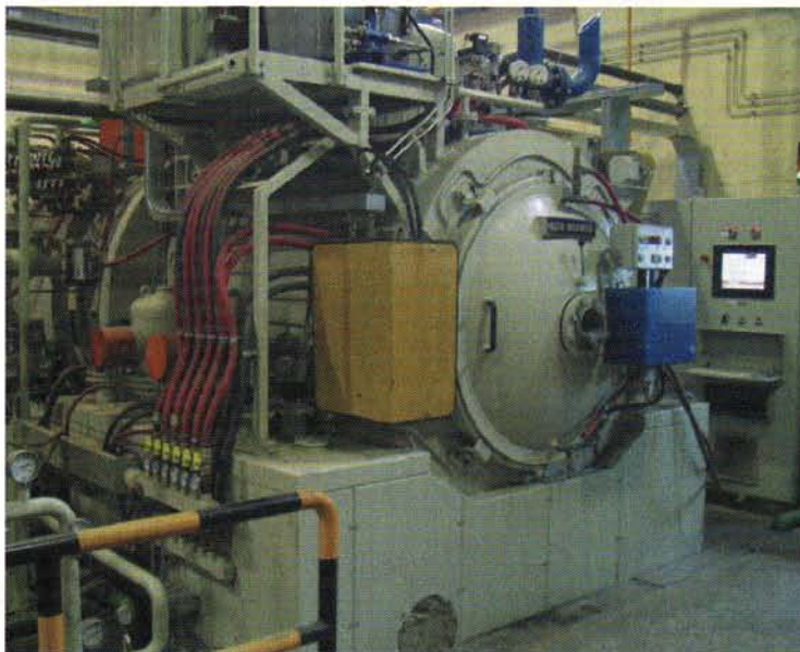
Fig. 12 — Double- chamber oil-quench furnaces 18 × 20 × 24 in. (top) and 30 × 24 × 48 in. (right) work chambers.
