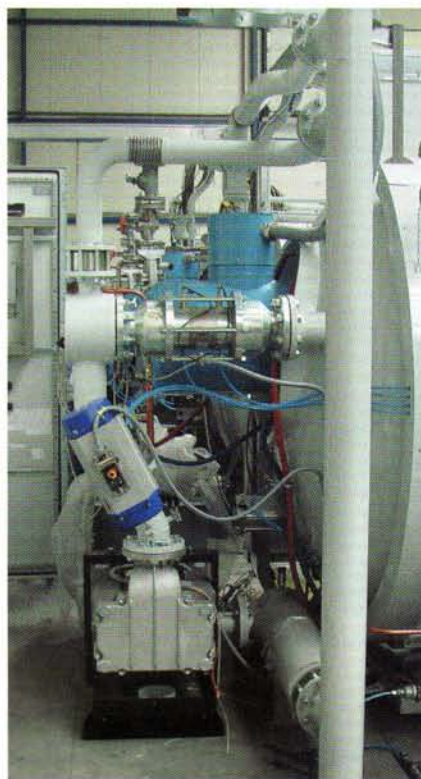
Fig. 8 - Pumping system for 25 bar hydrogen.
