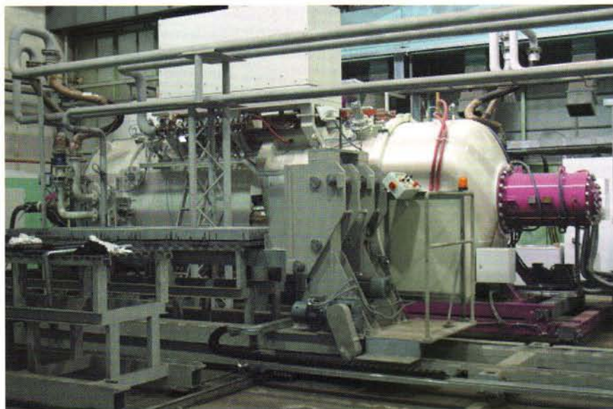
Fig. 4 — View of the 36 x 32 x 140 in. HPQ furnace
