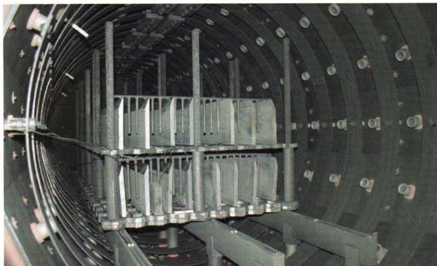
Fig. 3 — HPQ furnace with 36 x 32 x 140 in. work chamber designed for thermal treatment of knives (cutters) made of AISI S5 steel.
