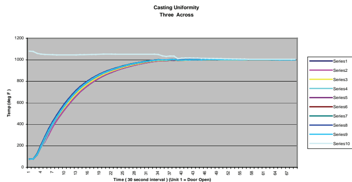
Fig. 6 Temperature vs. time for the complete test
