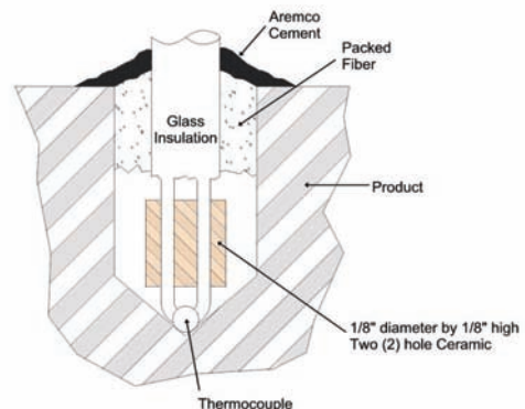
Fig. 4 Thermocouple Configuration
