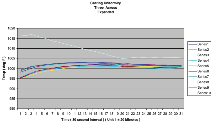
Fig. 7 Temperature vs. Time in an expanded scale beginning when all temperatures were above 995 deg. F
