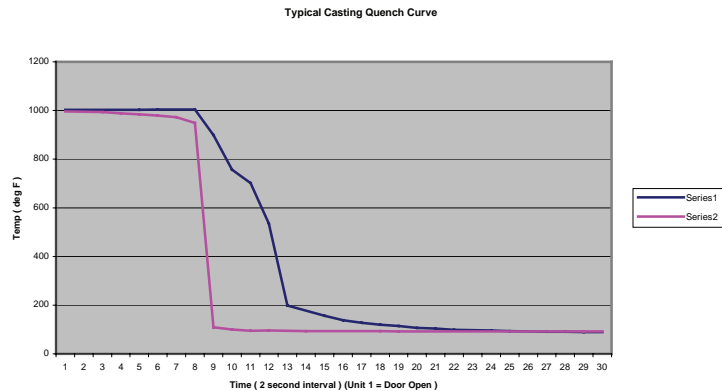
Fig. 10 Typical temperatures during the heat/hold portion of the heat treat cycle
