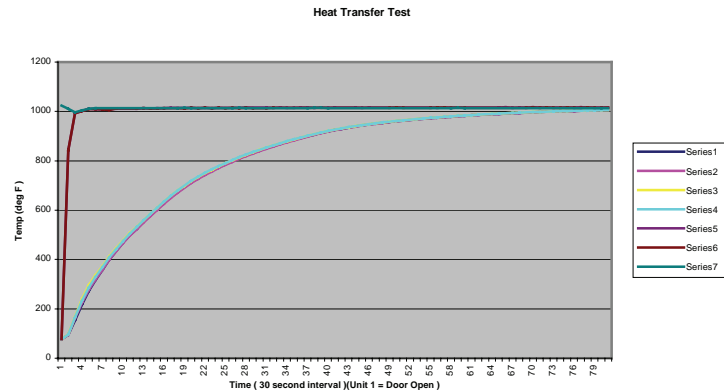
Fig. 8 Plate temperature vs. elapsed time (heating curve) for a one inch thick 6061 aluminum plate at a distance of 4-1/4 inches from the jet plate
