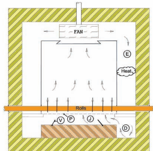
Fig. 1 Mass Flow – Jet Impingement Furnace
